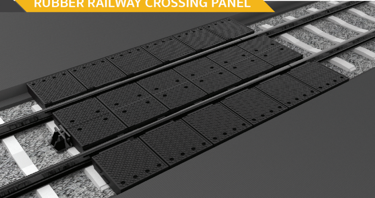
Rubber Railway Level Crossing Panel | Internal Dimension : 600 x 526.5 x 170 mm.
